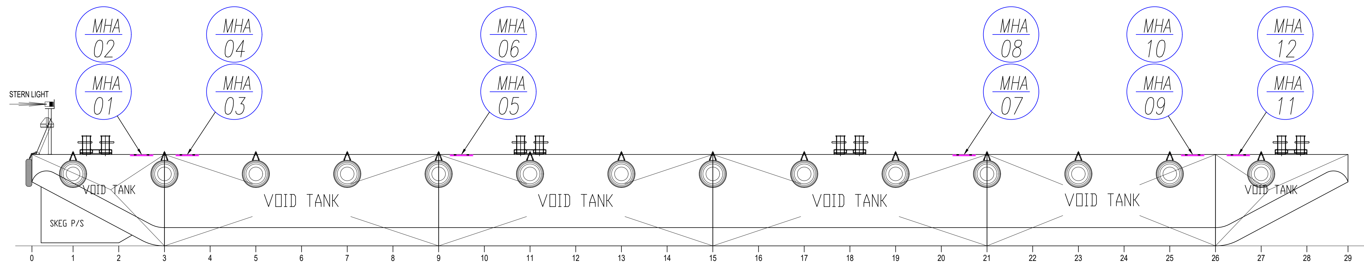
OUTBOARD PROFILE
